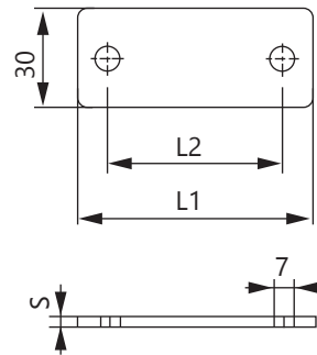
Cover plate
