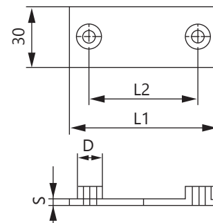
Welded base plate
