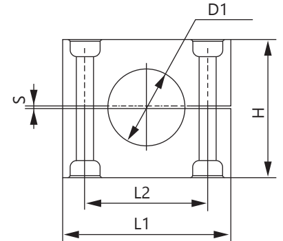
Clamp body
